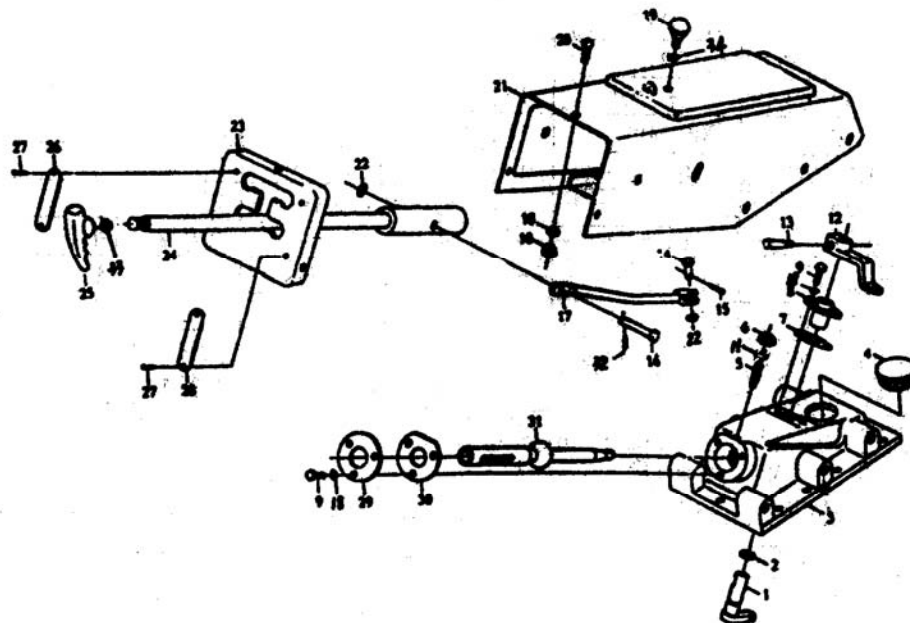
Fig.7 “Г” Shaped Gears Sub-transmission Control System Assembly
